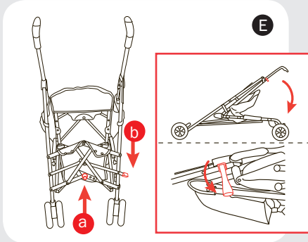
FIGURE E - FOLDING YOUR STROLLER
